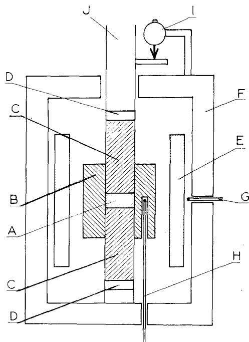
Figure 1 Hot-pressing cell (schematic). A, sample; B, die; C, pistons; D, thermal insulation; E, heating resistor; F, wall; G, regulating thermocouple; H, measuring thermocouple; I, displacement sensor; J, hydraulic ram.
