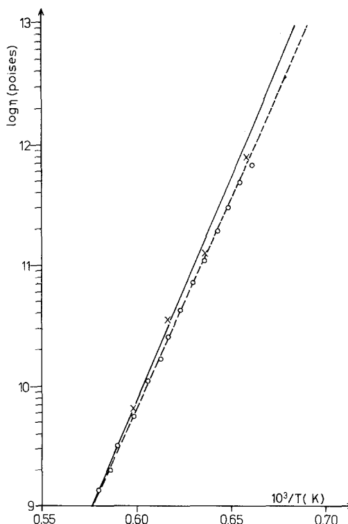
Figure 12 Viscosity of vitreous silica calculated from Murray et al. model \times - \times - \times isothermal \circ - \circ - \circ dynamic study; - data after [15].
